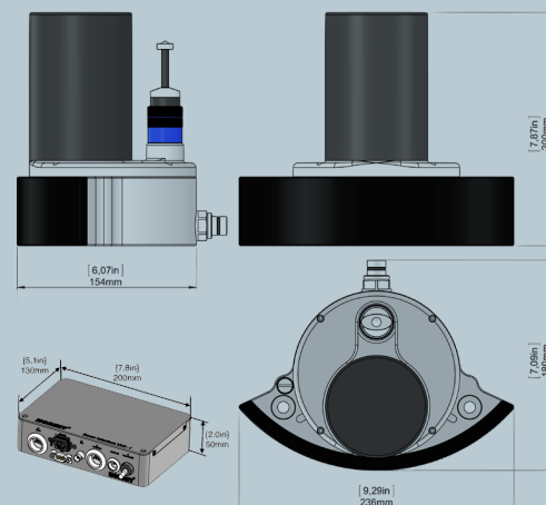
Dimensions shown for standard version
